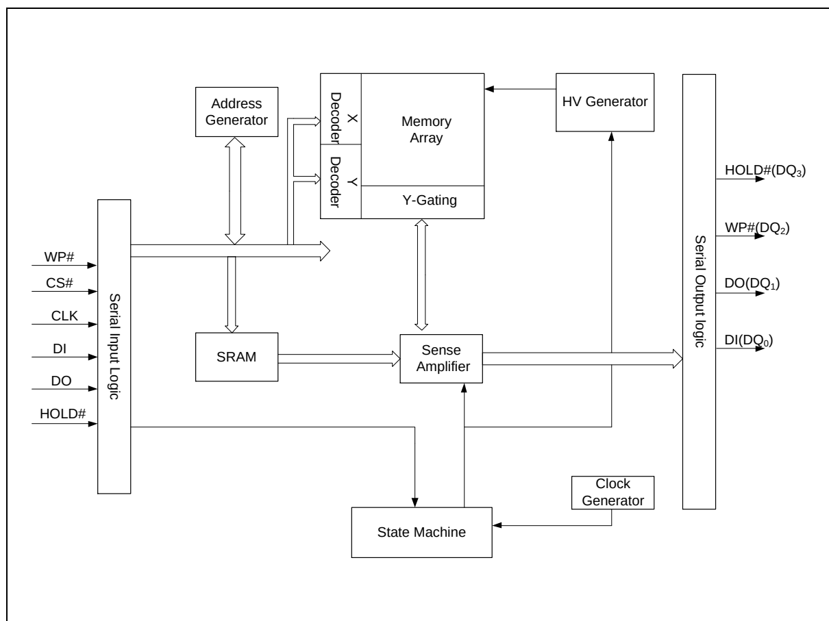
Figure 1 FM25LQ32I2 Serial Flash Memory Block Diagram
