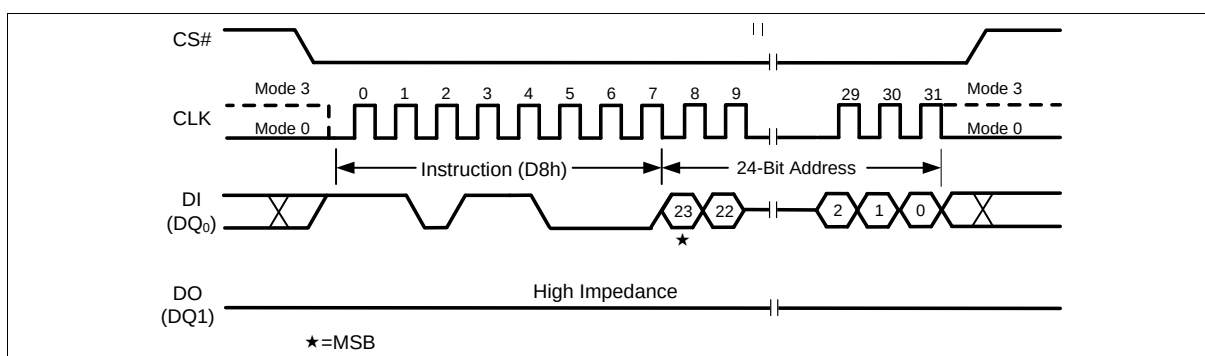
Figure 35 64KB Block Erase Instruction (SPI Mode)
