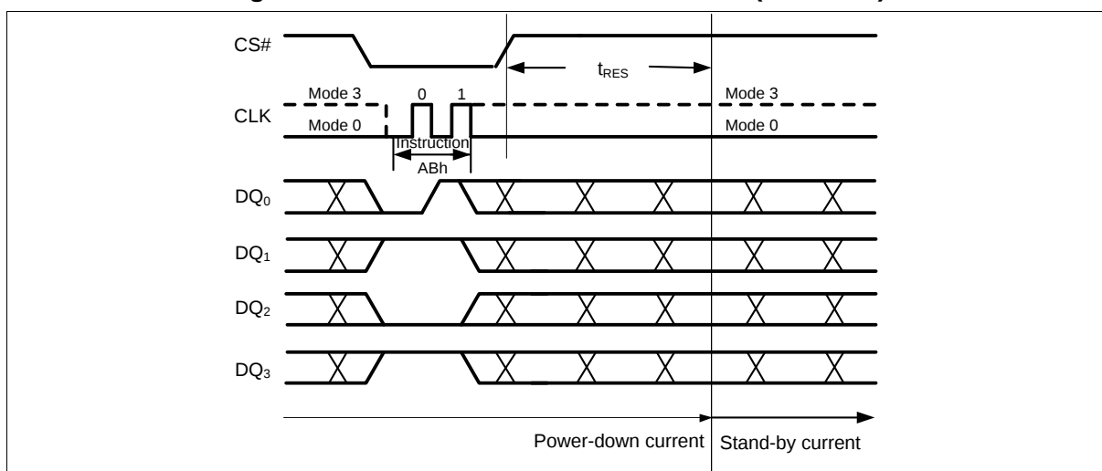
Figure 44 Release Power-down Instruction (SPI Mode)
