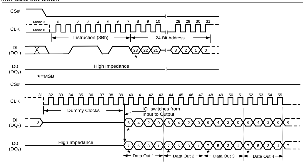
Figure 20 Fast Read Dual Output Instruction (SPI Mode only)
