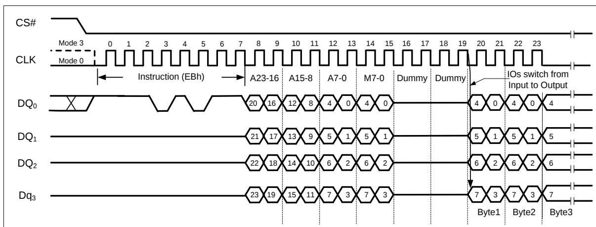
Figure 24 Fast Read Quad I/O Instruction (Initial instruction or previous M5-4#10, SPI Mode)
