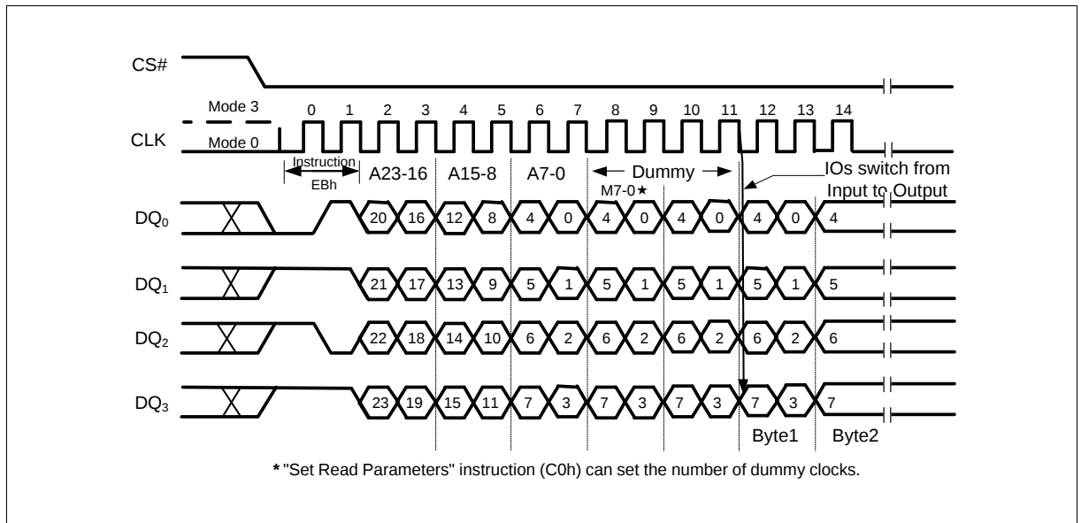
Figure 26 Fast Read Quad I/O Instruction (Initial instruction or previous M5-4#10, QPI Mode)
