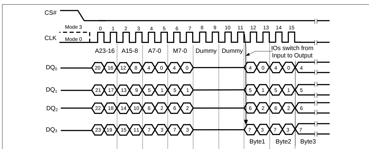
Figure 25 Fast Read Quad I/O Instruction (Previous instruction set M5-4 = 10, SPI Mode)
