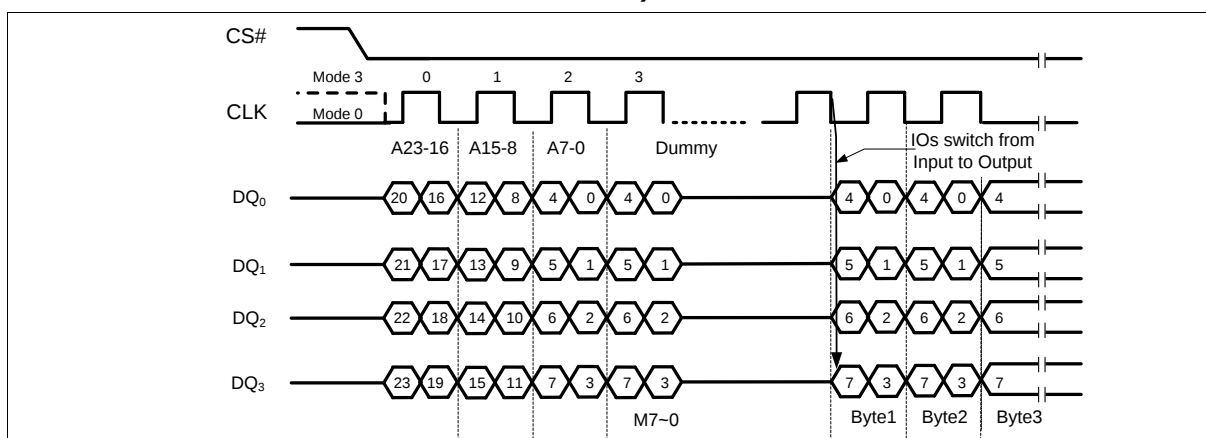
Figure 33 Fast Read Quad I/O Instruction (Previous instruction set M5-4 = 10, SPI Mode)
